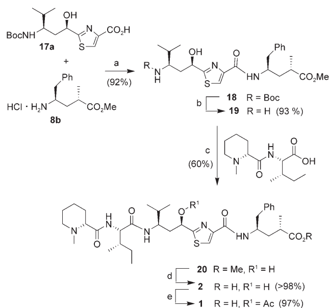
Scheme 5. Synthesis of tubulysins U and V. a) HOAt, HATU, TMP, DMF, 3 h; b) CH 2 Cl 2 , 20% TFA, 1 h; c) isoBuO 2 CCl, NMM, AcOEt, 8 h; d) LiOH, THF/H 2 O (4:1), 3 d, then TFA; e) Ac 2 O, Py, 14 h. HOAt = 7-aza-1-hydroxy-1 H -benzotriazole, HATU = N -[dimethylamino]-1 H -1,2,3-triazole[4,5- b ]pyridin-1-ylmethylen]- N -methylmethanaminium hexafluorophosphate, TMP = 2,4,6-trimethylpyridine, TFA = trifluoroacetic acid.
