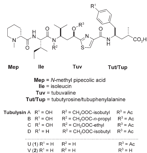
Scheme 1. Structure of tubulysins.
